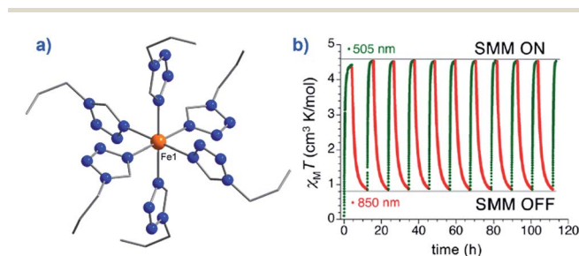
Fig. 8 (a) Molecular structure of [Fe(1-ptz) 6 ] 2 [(BF 4 ) 2 ] (2). Colour code: orange (Fe), blue (N), and grey (C). Hydrogen atoms omitted for clarity. (b) Excitation and de-excitation cycling between the HS and LS configuration of 2, represented as a variation in the \chi_M T product at 10 K, under a 5000 Oe field. Reprinted with permission from ref. 28. Copyright (2013) American Chemical Society.
