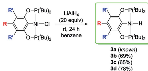
Scheme 4 Synthesis of the \text{tBu[POCOP]NiH} complexes.
