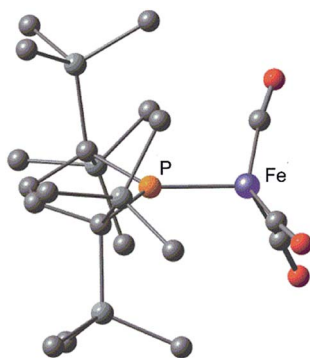
Fig. 5 DFT(PBE0) optimized structure of 3_{\text{opt}} .
