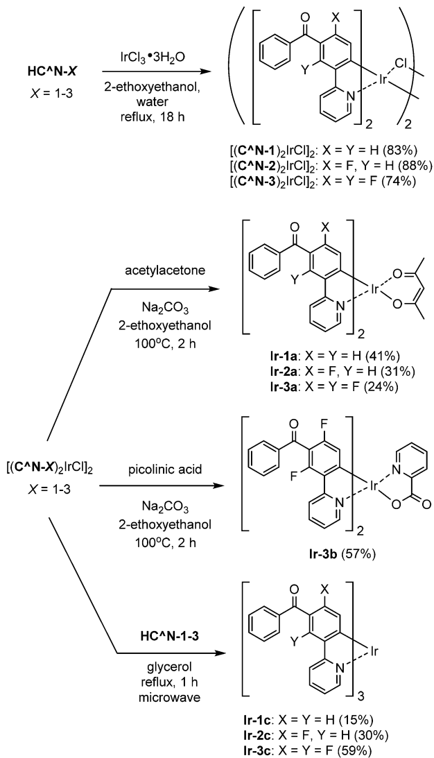
Scheme 2 Syntheses of iridium(III) complexes.
