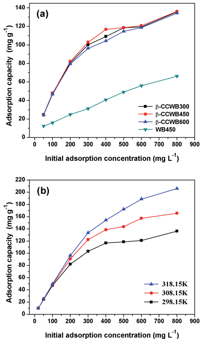
Fig. 4 (a) The comparison of adsorption capacity on \beta -CCWB and WB450 under 298.15 K, (b) the comparison of adsorption capacity on \beta -CCWB450 under different adsorption temperatures (Cr(vi) solution volume: 50 mL; adsorbent dose: 0.1 g; contact time: 24 h; pH: 2.0).
