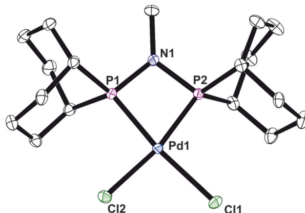
Fig. 6 Crystal structure of complex [\text{PdCl}_2(\text{L}_e)] ( 6 ). All hydrogen atoms have been omitted for clarity. Selected bond lengths ( \text{\AA} ) and angles ( ^\circ ); Pd(1)–P(1) 2.2311(4), Pd(1)–P(2) 2.2353(4), Pd(1)–Cl(2) 2.3735(4), Pd(1)–Cl(1) 2.3748(4), P(1)–N(1) 1.6949(14), P(2)–N(1) 1.7016(14), P(1)–Pd(1)–P(2) 70.851(15).
