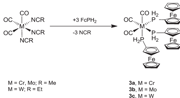
Scheme 3 Synthesis of fac - [M(CO)_3(PH_2Fe)_3] ( 3a , M = Cr ; 3b , M = Mo ; 3c , M = W ).
