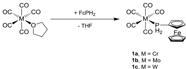
Scheme 1 Synthesis of [M(CO)_5(PH_2Fe)] ( 1a , M = Cr ; 1b , M = Mo ; 1c , M = W ).
