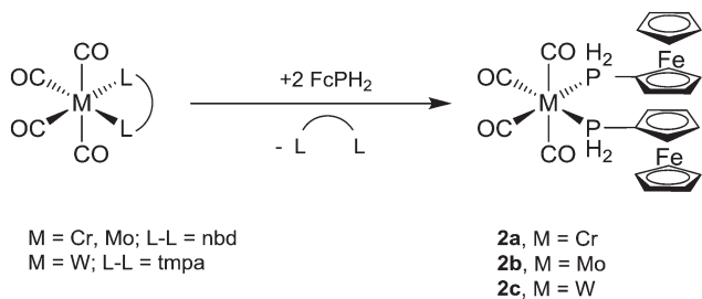
Scheme 2 Synthesis of cis - [M(CO)_4(PH_2Fe)_2] ( 2a , M = Cr ; 2b , M = Mo ; 2c , M = W ).
