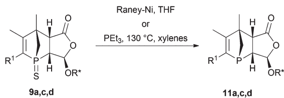
Scheme 2 Desulfurisation of P-chiral 1-phosphanorbornenes; yields and conditions: endo - 11a : 55%, Raney nickel; endo - 11c : 75%, Raney nickel; exo - 11c : 87%, Raney nickel; endo - 11d : 93%, \text{PET}_3 ; exo - 11d : 71%, Raney nickel.
