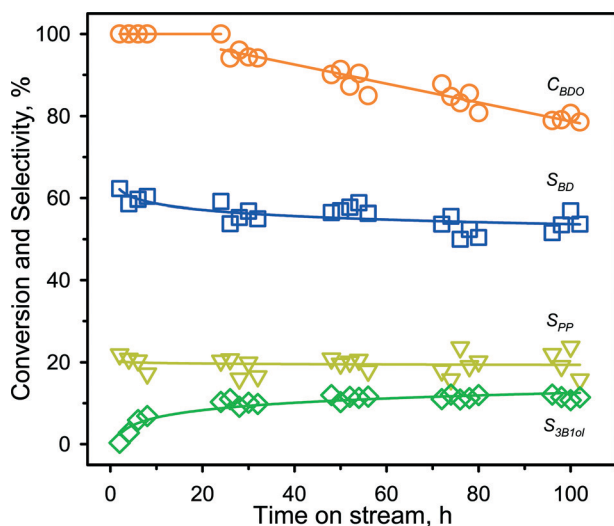
Fig. 2 Catalytic stability over ZSM-5@260 at 300 °C. Reaction conditions: T , 300 °C; ambient pressure, catalyst loading, 200 mg; liquid flowrate, 2.8 \text{mL h}^{-1} ; carrier gas flowrate, 60 \text{mL (STP) min}^{-1} . Nomenclature: C_{\text{BDO}} , 1,3-BDO conversion; S_{\text{BD}} , selectivity to BD; S_{\text{PP}} , selectivity to PP; S_{\text{3B1ol}} , selectivity to 3-buten-1-ol.
