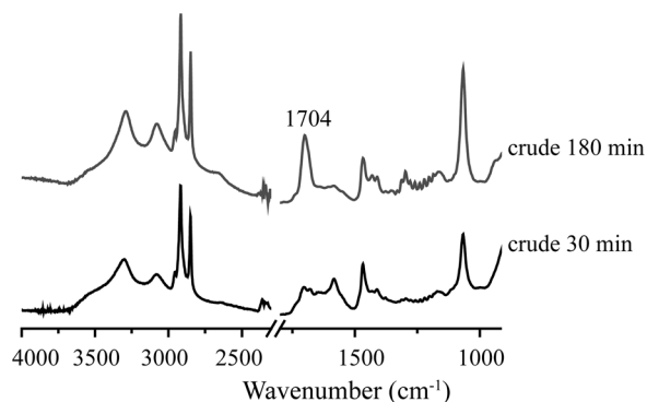
Fig. 9 ATR-IR spectra of a spent Pt/Al 2 O 3 catalyst after crude glycerol APR; after 30 min and after 180 min.
