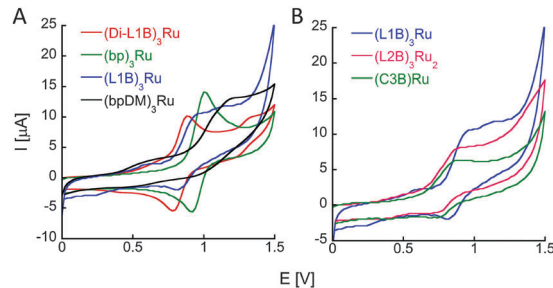
Fig. 3 Comparison between the cyclic voltammograms of (A) 0.5 mM intermolecular \text{Ru} complexes and (B) 0.5 mM (L1B) 3 Ru and (C3B)Ru and 0.25 mM (L2B) 3 Ru 2 that were recorded in acetonitrile at rt. using a glassy carbon working electrode, platinum counter electrode, and \text{Ag}/\text{AgNO}_3 reference electrode. Scan rate: 100 \text{mV s}^{-1} .
