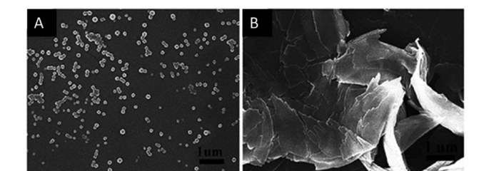
Fig. 34 Schematic representation of the anion- \pi induced self-assembly forming the vesicle as well as SEM images before (A) and after addition of 3 eq. of \text{NaNO}_3 (B). Reproduced with permission from John Wiley and Sons. 66
