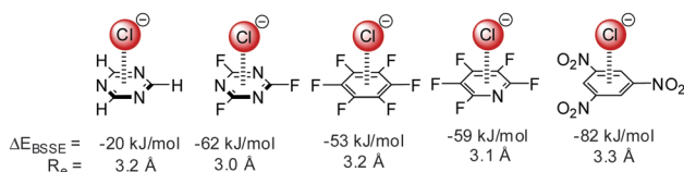
Fig. 2 Interaction energy with basis set superposition error correction ( E_{\text{BSSSE}} ) and equilibrium distances ( R_e ) of selected anion- \pi complexes from the MP2/6-31++G** level of theory. 7,15,16
