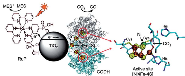
Fig. 19 Schematic illustrating the CODH 1 modified and Ru dye-sensitized TiO 2 NPs photoactive system. Reprinted with permission from ref. 176. Copyright 2010 American Chemical Society.
