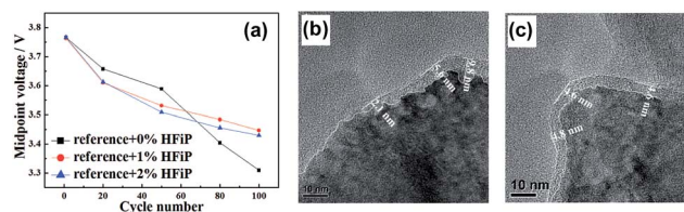
Fig. 24 Midpoint voltage of cells at a current density of 180 mA g -1 in the voltage range of 2.0–4.6 V with electrolytes containing 0%, 1% and 2% HFiP additive. TEM images of \text{Li}[\text{Li}_{0.2}\text{Mn}_{0.56}\text{Ni}_{0.16}\text{Co}_{0.08}]\text{O}_2 cathodes in the electrolyte (b) without and (c) with HFiP additive at 18 mA g -1 after 1 cycle. Reproduced with permission. 115
