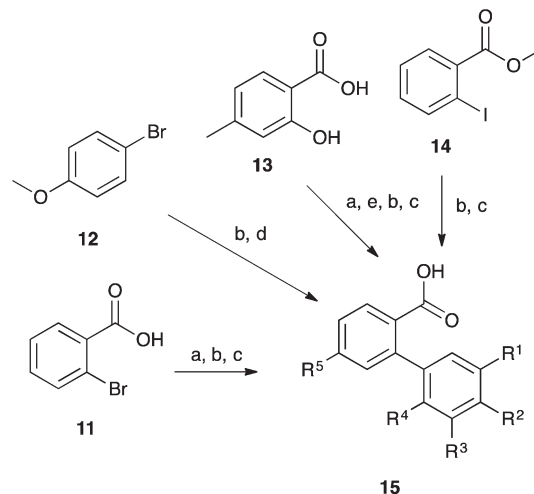
Scheme 4 The formation of the substituted biphenyl carboxylic acids 15 . (a) cat. H 2 SO 4 , MeOH, \Delta ; (b) ArB(OH) 2 , SPhos, Pd(OAc) 2 , Na 2 CO 3 , CH 3 CN/H 2 O, \Delta ; (c) NaOH, EtOH, \Delta , then acid work-up; (d) KMnO 4 , Py/H 2 O, \Delta ; (e) Tf 2 O, NEt 3 , DCM, 0 °C.
