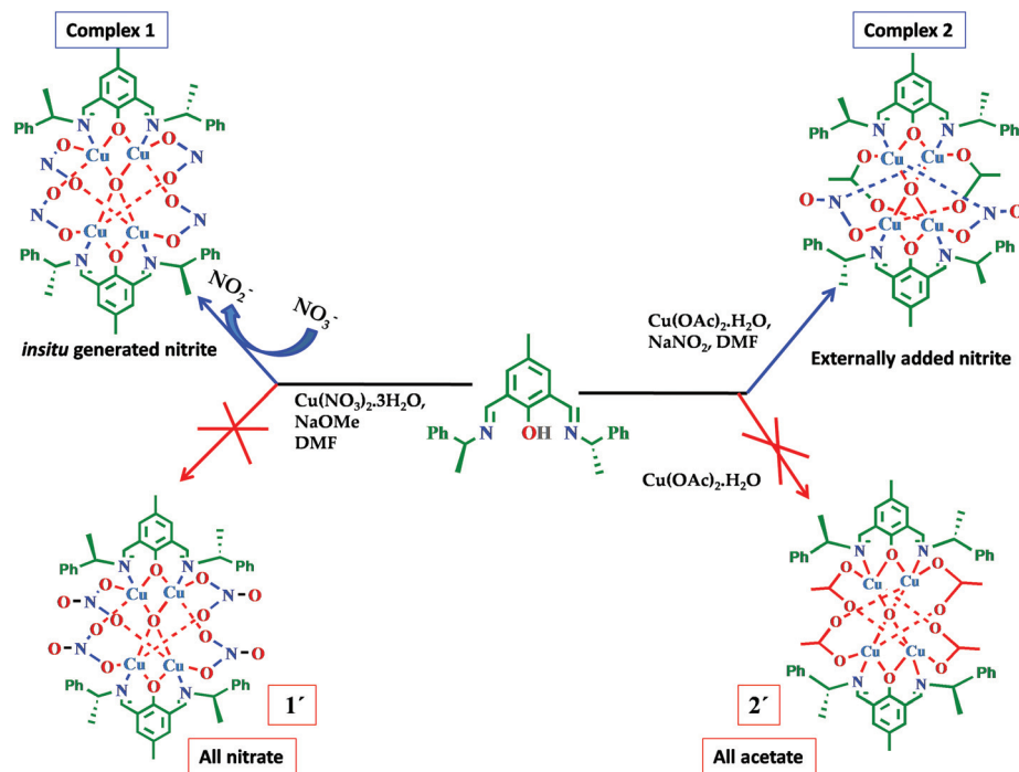
Scheme 2 Synthesis of the complexes.
