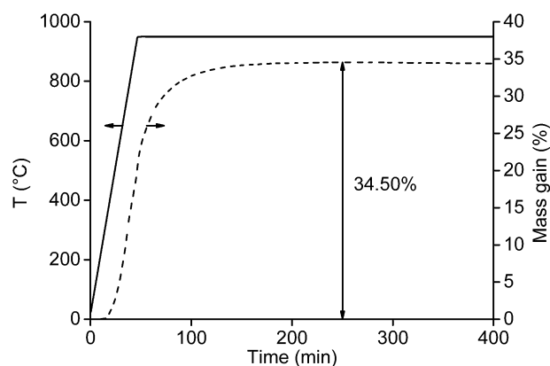
Fig. 2 Thermogravimetric analysis of the magnet powder <400 \mu\text{m} . The NdFeB magnet powder was first heated to 950 °C (heating rate: 20 °C \text{min}^{-1} ) and kept at this temperature for another 6 h. The temperature of the furnace is given by the solid line and the mass gain (%) by the dashed line.
