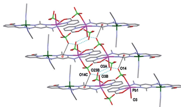
Fig. 6 View of the arrangement of complex 1 into a one dimensional chain in the [1\ 0\ 0] direction through H-bonding. The anion- \pi interaction between O14 and the central pym rings is also shown (hydrogens have been omitted for clarity; symmetry codes (A) -1 + x, y, z ; (B) -x, 1 - y, -z ).
