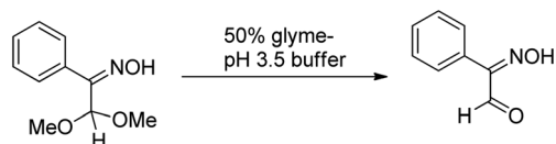
Scheme 30 Hydrolysis of phenylglyoxal dimethyl acetal oxime.
