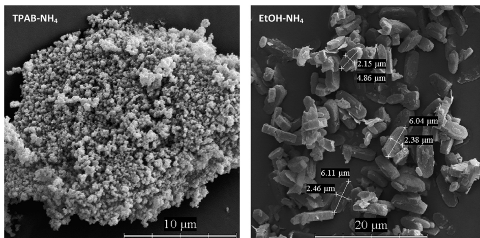
Fig. 1 SEM images of the studied ZSM-5 zeolites.
