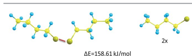
Fig. 6 Conformation and energy difference of dibutyl disulfide and the product obtained when the disulfide bond (red) is broken homolytically.
