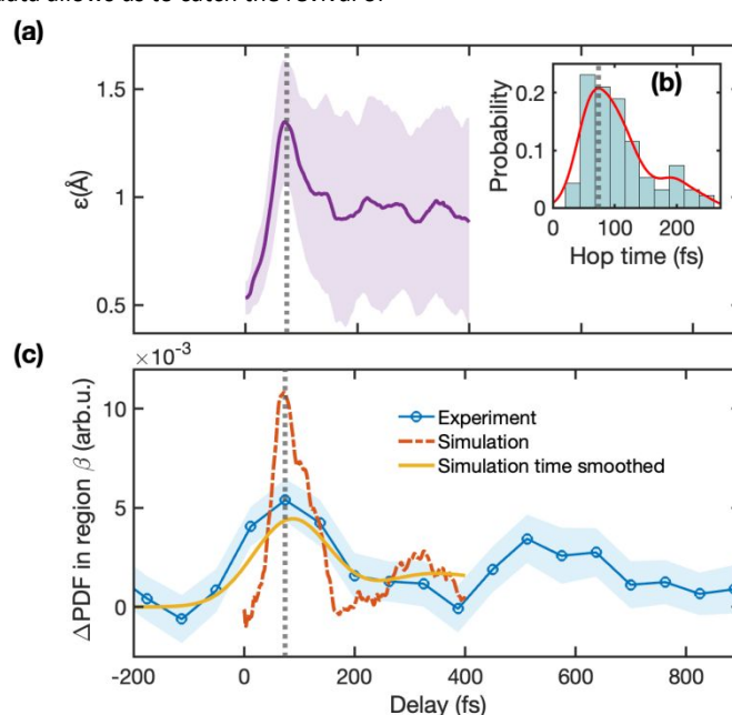
Figure 6: Ring stretching motion dynamics reflected in the experiment and simulated \Delta PDF s. Panel (a) shows the amount of ring stretching averaged over the simulated trajectories as a function of time delay ( \varepsilon_{avg}(t) ) along with the standard deviation from the mean. The inset (b) shows the probability distribution of hop times from S_1 to S_0 (excited-state to ground-state) for all trajectories. Panel (c) shows the sum of \Delta PDF intensity in the region \beta ( 2.6 < r(\text{\AA}) < 3 ) for the experiment (blue) along with the one-standard-deviation error (shaded region), the corresponding signal from the simulation without (red) and with (yellow) 150 fs gaussian time smoothing applied. The vertical grey dotted line in Panels (a), (b), and (c) marks the most likely time (74 fs) for the wavepacket to reach the CI seam.
