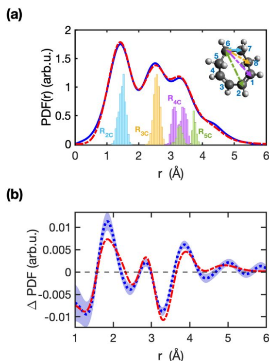
Figure 2: Comparison of experimental and simulated diffraction signals in real space. Panel (a) shows the experimental (blue-solid line) and simulated (red dashed line) stationary ground-state PDF( r ) of COD. The blue, yellow, purple, and green histograms in panel (a) depict the distribution of carbon-carbon distances of the geometries in the TSH simulations at time-zero, for the ground-state Wigner ensemble. The inset illustrates the averaged stationary-ground state molecular structure (at T = 0 fs) with different carbon-carbon distances marked in color code for one of the carbon atoms in the molecule ( R_{2C} , R_{3C} , R_{4C} , and R_{5C} distances are marked in blue, yellow, purple, and green arrows, respectively). Panel (b) shows the experimental (dotted blue line) and simulated (dashed red line) \Delta PDF averaged over delays between 250 fs to 400 fs. The shaded blue area in panel (b) represents the statistical one-standard deviation error of the experiment signals calculated from a bootstrap analysis.
