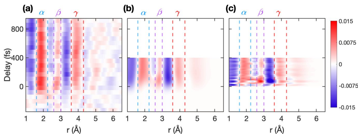
Figure 3: Experiment and simulated \Delta PDFs. The false color plots show the difference diffraction signal ( \Delta PDF ( r , t )) in real space as the function of pump-probe delay for (a) experiment, (b) (scaled) simulation convolved in time with a Gaussian of 150 fs full width at half maximum (FWHM), and (c) (scaled) simulation without any convolution in time. The regions \alpha ( 1.6 < r(\text{\AA}) < 2.25 ), \beta ( 2.6 < r(\text{\AA}) < 3 ), and \gamma ( 3.6 < r(\text{\AA}) < 4.3 ) are marked in all three panels with blue, purple, and red broken lines, respectively. The \Delta PDF in region \beta ( 2.6 < r(\text{\AA}) < 3 ) has a modulation in intensity with the delay.
