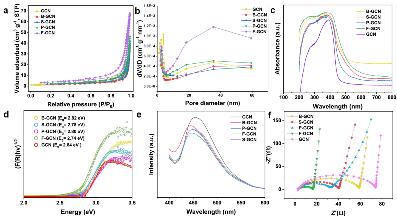
Fig. 4 (a) N_2 adsorption-desorption isotherms of GCN and non-metal doped GCN, measured volumetrically at -196^\circ\text{C} . (b) Pore size distribution curves of GCN and non-metal doped GCN. (c) UV-vis diffuse reflectance spectra and (d) Kubelka-Munk plots for band gap estimation of GCN and non-metal doped GCN. (e) Steady-state PL spectra and (f) EIS spectra of GCN and non-metal doped GCN.
