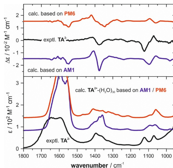
Fig. 8 Comparison of the experimental VCD and IR spectra of \text{TA}^{2-} with the computed spectra obtained by averaging \text{TA}^{2-}-(\text{H}_2\text{O})_{30} clusters extracted from MD simulations at the AM1/TIP3P and PM6/TIP3P levels of theory.
