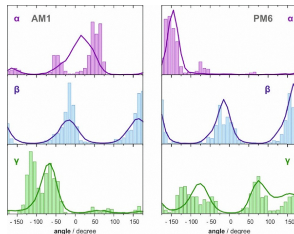
Fig. 7 Histograms showing the torsional angle distributions extracted from QM/MM-MD trajectories at the AM1 and PM6 levels (solid lines) compared to optimized conformers \text{TA}^{2-}-(\text{H}_2\text{O})_{30} (bars).
