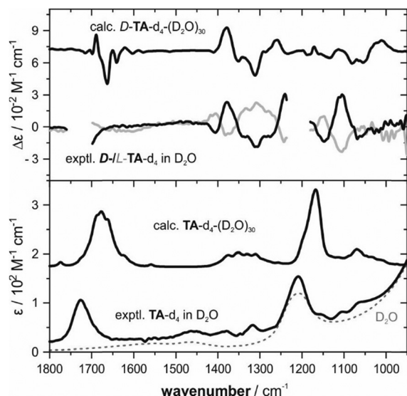
Fig. 6 Comparison of the experimental VCD and IR spectra of TA in \text{D}_2\text{O} with the computed spectra obtained by averaging \text{TA-d}_4-(\text{D}_2\text{O})_{30} clusters extracted from MD simulations at the AM1/TIP3P level of theory.
