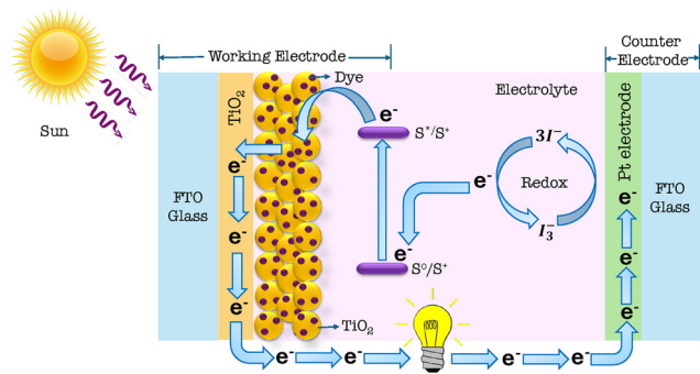
Fig. 1 Schematic diagram illustrating the working principle of a DSSC.
