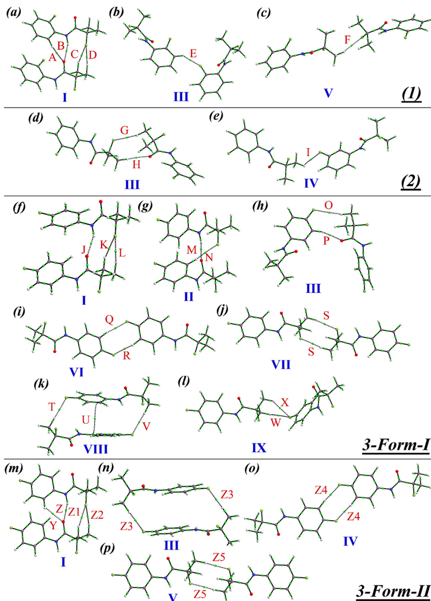
Fig. 9 Distribution of bond critical points (BCP) and bond paths of intermolecular interactions in the molecular pairs involving C–H⋯F interactions in (a–c) 1 , (d and e) 2 , (f–l) 3-form-I , and (m–p) 3-form-II , respectively.
