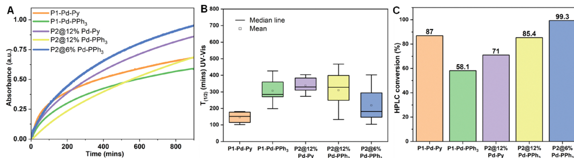
Fig. 2 (A) Kinetic profiles of encapsulated P1 and covalently attached P2 NPs in a pro-DNP (4) (100 μM) to DNP (5) conversion monitored by UV-Vis over time at λ = 400 nm in water at 37 °C using 30 μM of Pd; (B) T 1/2 comparison of the P1 and P2 NPs in the formation of DNP (5); T 1/2 (time taken for 50% formation of DNP (5) by UV-Vis, mean of multiple runs); (C) HPLC conversion of DNP (5) after 24 h.
