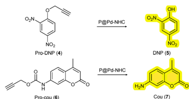
Scheme 2 Model prody activation using Pd nanoparticles.
