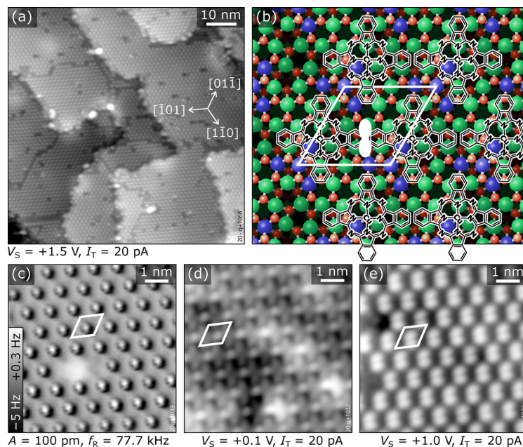
Fig. 5 The (1 \times 1) superstructure of CuPc/In 2 O 3 (111). (a) Overview STM image showing the three distinct orientational domains separated by domain boundaries (dark lines). Dark dots within the domains are missing molecules. (b) Sketch of the In 2 O 3 (111) substrate superimposed with the structure of CuPc molecules in the (1 \times 1) arrangement (one rotational domain is shown). The unit cell of the structure is indicated in white and the white double-lobed area indicates the overlap of neighboring molecules leading to maxima in the STM images. (c) nc-AFM image of an area with a single CuPc missing. The protrusions forming a (1 \times 1) pattern are benzene rings bent away from the surface; the macrocycle of the molecule is not visible. (d) and (e) Empty-states STM images of the same rotational domain as in (c), but taken in an area without a CuPc vacancy. Panel (d) was acquired at a bias voltage below the CuPc LUMO; the cross-like features are individual CuPc molecules. The overlapping benzene rings of neighboring molecules are brighter than the rest of the molecule. Panel (e) displays the same surface area as (d) but at the energy of the LUMO. The bright double-lobed features originate from the LUMO at the benzene rings bent upwards, as also indicated in panel (b). All images were acquired at 5 K.
