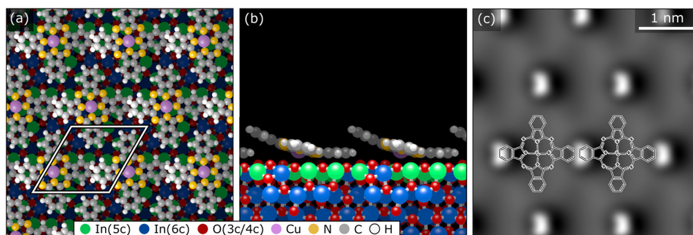
Fig. 6 Densely packed (1 \times 1) layer of CuPc on In 2 O 3 (111). (a) Top view of the DFT-optimized geometry. (b) Side view of the DFT-optimized geometry. Note that only a single row of molecules is shown to clearly display the distortion of the molecules due to the steric hindrance between the benzene rings of neighboring molecules. (c) Simulated constant-height AFM image using the probe-particle model. Only the protruding parts of the molecules are visible.
