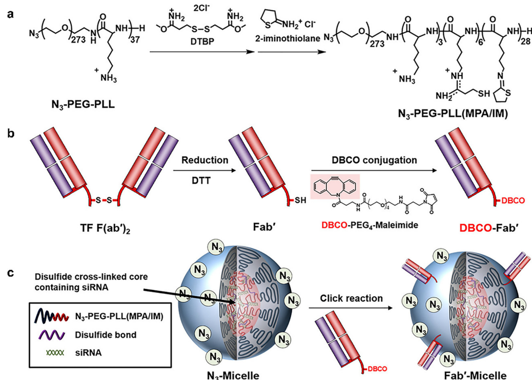
Fig. 13 Schematic illustration of Fab'-micelle construction. (a) The synthesis scheme of azide-functionalized block cationomer. (b) Preparation scheme of DBCO-Fab'. (c) DBCO-Fab' installation to N3-micelle. Reproduced with permission. 286 Copyright 2018, American Chemical Society.
