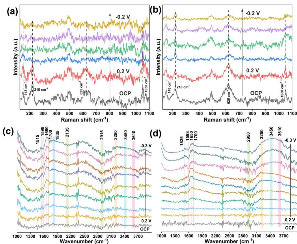
Fig. 6. In-situ Raman spectra of (a) \text{Cu}_2\text{O}/\text{Cu-R} and (b) Pt- \text{Cu}_2\text{O}/\text{Cu-R} for the \text{NO}_3\text{RR} at different potentials; In-situ FTIR spectra of (c) \text{Cu}_2\text{O}/\text{Cu-R} and (d) Pt- \text{Cu}_2\text{O}/\text{Cu-R} for the \text{NO}_3\text{RR} at different potentials.
