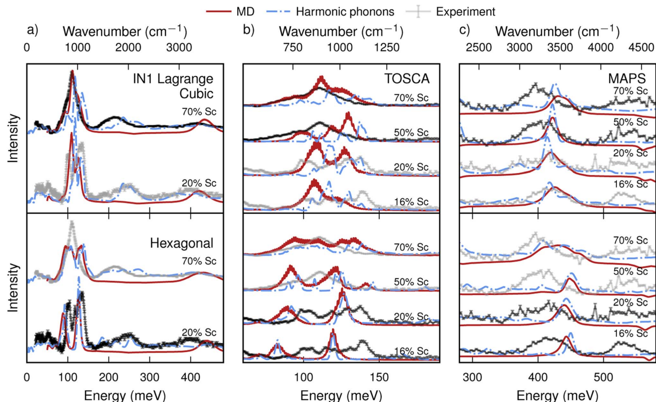
Fig. 6 Hydrogen dynamics in hydrogenated Sc-doped \text{BaTiO}_3 ( \text{BaTi}_{1-x}\text{Sc}_x\text{O}_{3H_x} ) for various concentrations of dopants, compared with experimental results measured at three different neutron spectrometers: IN1 Lagrange, TOSCA, and MAPS. Experimental data are from ref. 58. (a) IN1 Lagrange is a wide-range spectrometer that probes the dynamics in the region from 0 to 500 meV. (b) TOSCA and (c) MAPS on the other hand can be used to study the region around 100 meV and 500 meV, respectively, utilizing the higher energy resolution they offer. Simulated spectra using our workflow (labeled MD) corrected for quantum statistics and the kinematic constraint of the specific instrument are shown for all concentrations of dopants considered experimentally, with the simulated structure both in the cubic and hexagonal structure. Experimentally, only one of these phases is stable for a given concentration of Sc, but the energy of the two phases are sufficiently close that both phases are stable on the timescales of the MD simulations. The experimental data has thus been duplicated in the upper and lower rows of plots, where the compositions that are stable for each phase are indicated by the black lines. Additionally, simulated spectra based on harmonic phonons obtained via AbINS are included for comparison.
