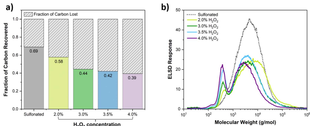
Fig. 2 (a) Fraction of carbon recovered as dissolved carbon by TOC relative to the total \text{H}_2\text{O}_2 concentration added in the Fenton reaction. (b) Molecular weight distributions after Fenton reaction as a function of \text{H}_2\text{O}_2 added starting from 2% at which point nearly all the material was soluble.
