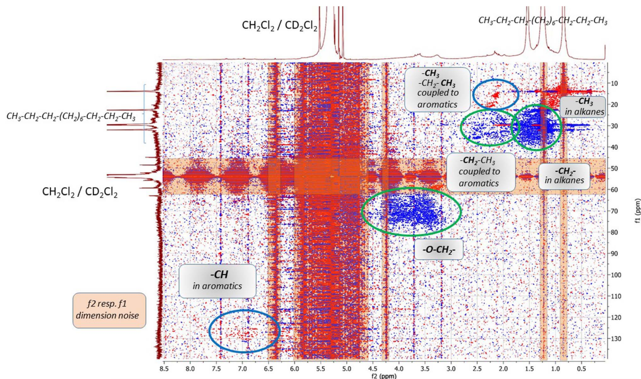
Fig. 13 2D ^{13}\text{C} , ^1\text{H} -correlated NMR spectrum (HSQC) of the organic extract of the soluble carbonaceous species, recorded with \text{CD}_2\text{Cl}_2 (ca. 1 : 1 mixture).
