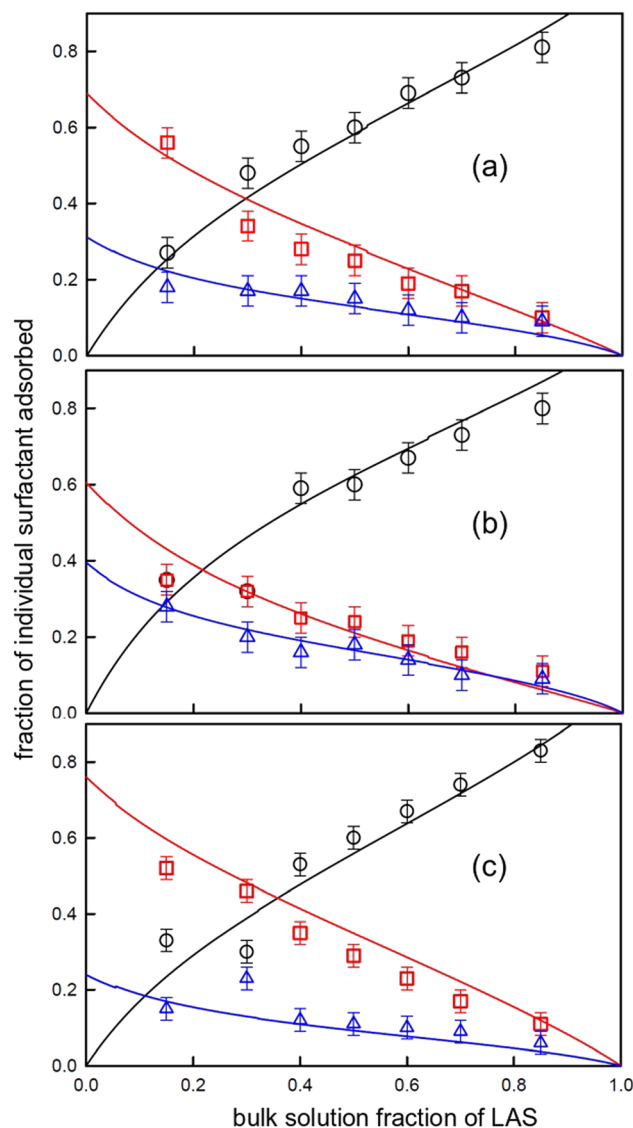
Fig. 3 Variation in adsorbed mole fraction with bulk mole fraction of LAS, for each of the ternary mixtures (a) LAS/2 : 1 R1/R2, (b) LAS/1 : 1 R1/R2, and (c) LAS/1 : 2 R1/R2, using data from ref. 58. The data points are (black) LAS, (red) R1, and (blue) R2, and the solid lines are calculated curves using the parameters in Table 2.
