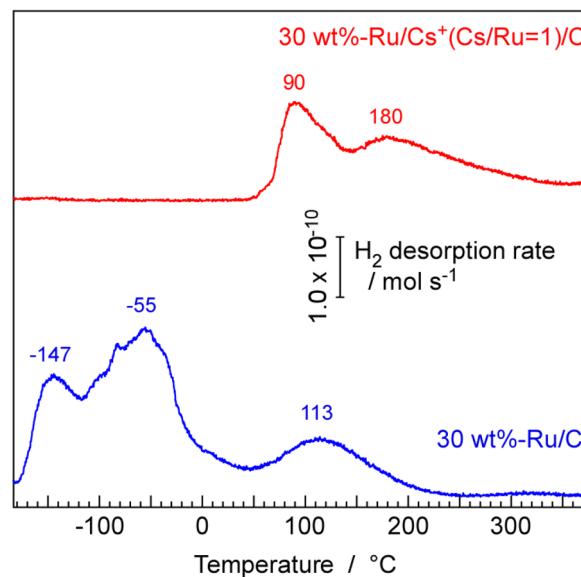
Fig. 10 TPD spectra of H 2 from 30 wt%-Ru/C and 30 wt%-Ru/Cs + (Cs + :Ru = 1:1)/C. The ramping rate of temperature was 10 °C min -1 . The samples were treated by reduction treatment at 400 °C, followed by evacuation at 400 °C, prior to TPD measurements. The adsorption of H 2 was performed at -183 °C and 5.0 kPa.
