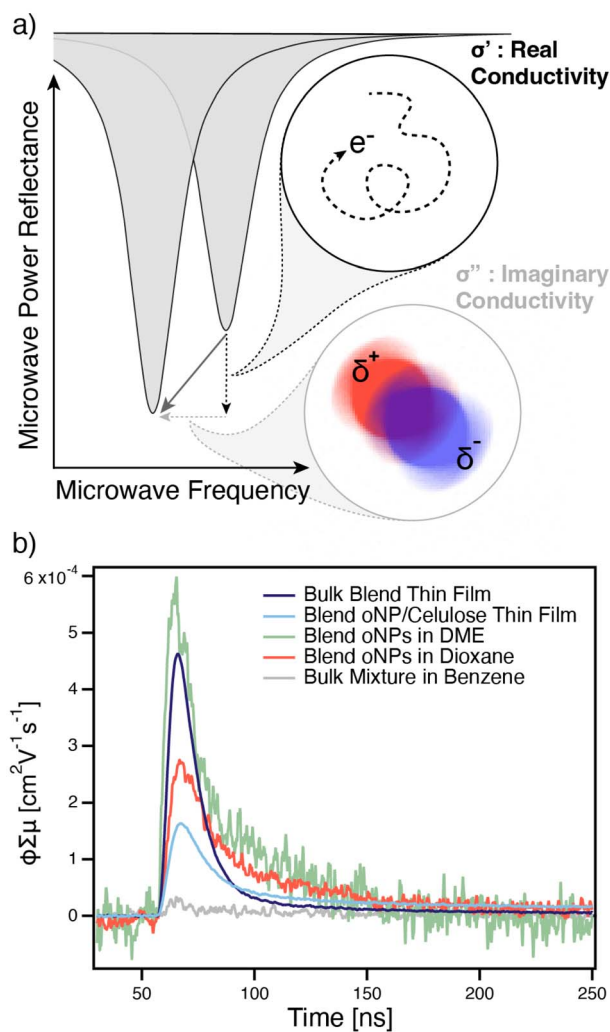
Fig. 7 (a) Schematic of concepts describing time-resolved microwave conductivity (TRMC) spectroscopy. Changes in depth ( y ) of the cavity's microwave resonance describe the diffusion of free charges (real conductivity, \Delta\sigma' ), while changes in frequency ( x ) of the cavity's microwave resonance describe changes in polarizability (imaginary conductivity, \Delta\sigma'' ); (b) TRMC transients corresponding to changes in real conductivity ( \Delta\sigma' ) for PTB7-Th : N2200 blend oNPs cast from water as a cellulose thin film (light blue trace), a PTB7-Th : N2200 bulk blend thin film (dark purple trace), PTB7-Th : N2200 blend oNPs in 1,4-dioxane (red trace), PTB7-Th : N2200 blend oNPs in DME (green trace), and a 1 : 1 mixture of bulk PTB7-Th + bulk N2200 in benzene (gray trace).
