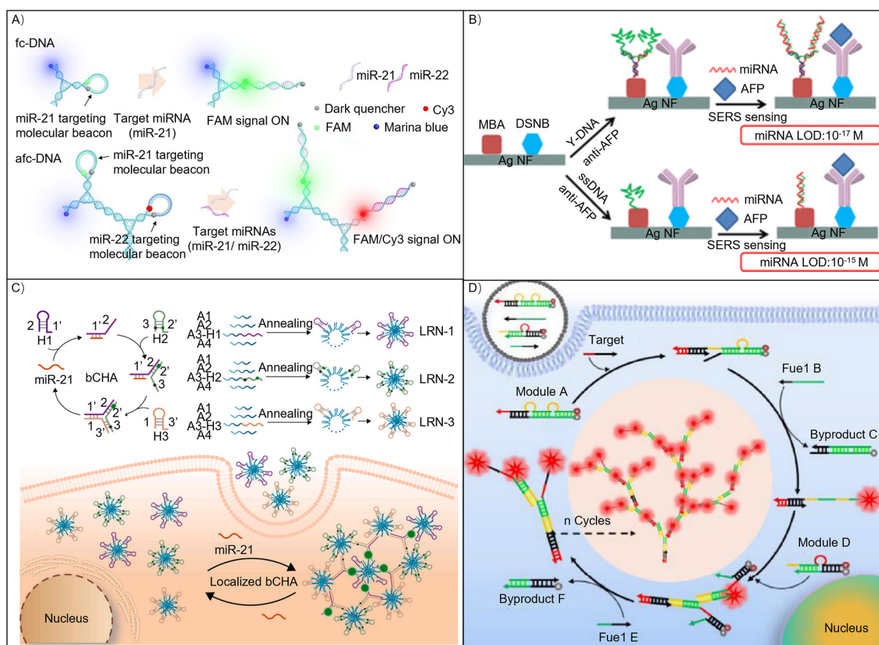
Fig. 5 (A) Branched DNA nanomaterials with fluorescent dyes for intracellular miR-22 and miR-21 detection. 171 (B) Branched DNA-based AgNP for detecting AFP and miRNA on SERS. 176 (C) Synthesis of branched DNA nanomaterials for miR-21 detection in living cells. 178 (D) Schematic diagram of target triggered synthesis of DNA dendrimers for contrast-increased imaging of miRNA in living cells. 179
