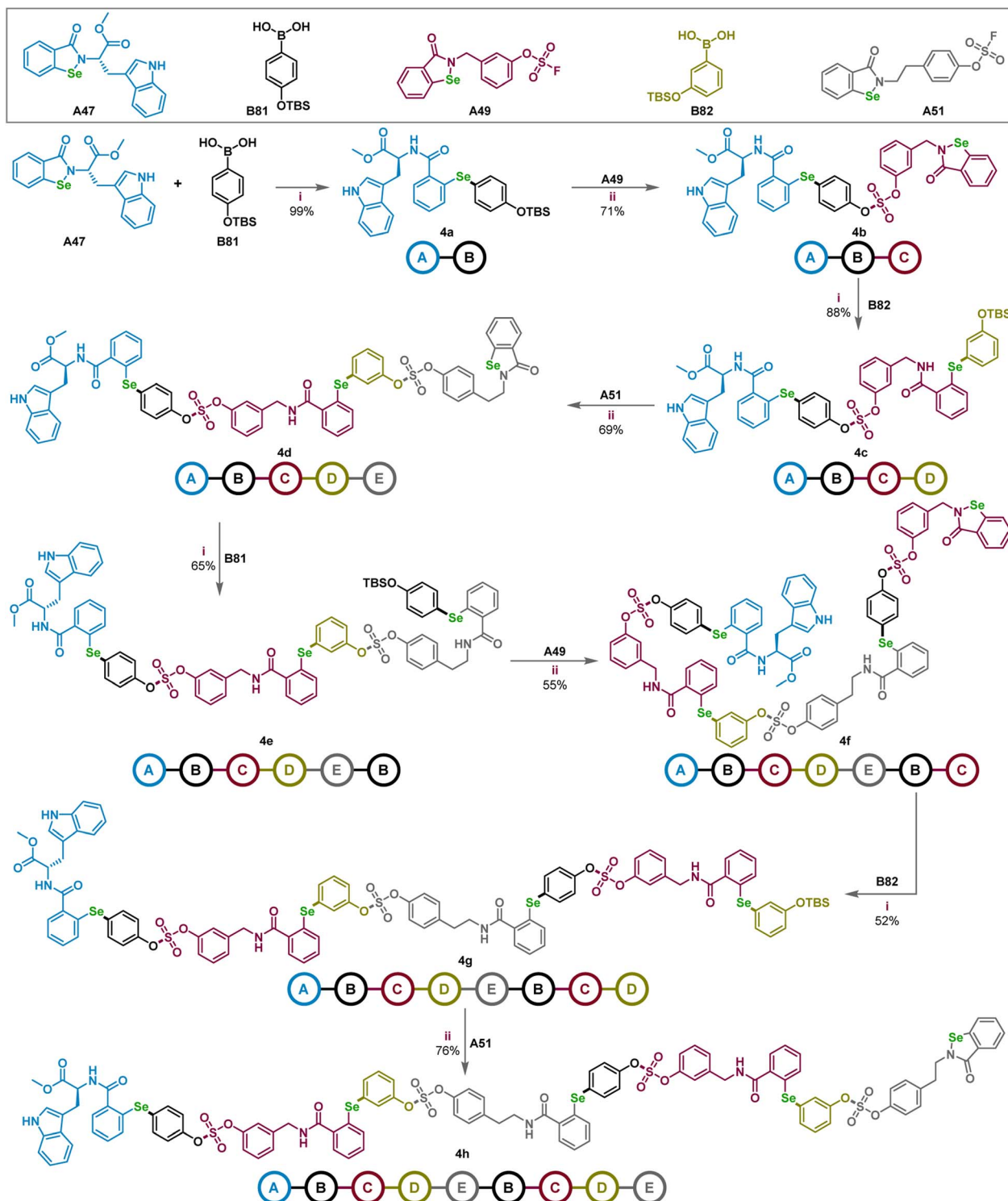
Fig. 4 Iterative SeNEx and SuFEx chemistries for the synthesis of sequence-defined oligo selenides. (i) SeNEx condition (a): BSEA (1.0 equiv.), boronic acid (1.2 equiv.), DIPEA (1.5 equiv.), \text{AgNO}_3 (5 mol%), EA, and rt. (ii): reactants (1.0 equiv.), 1,8-diazabicyclo-(5.4.0)undec-7-ene (DBU, 0.25 equiv.), MeCN, and 80 °C.
