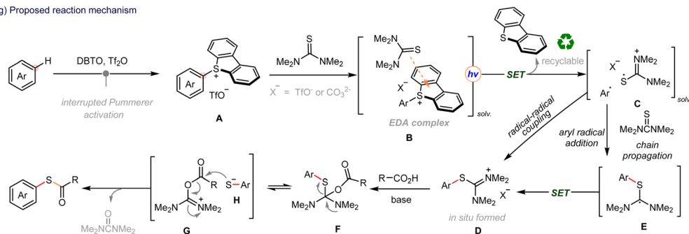
Scheme 3 Mechanistic studies.
