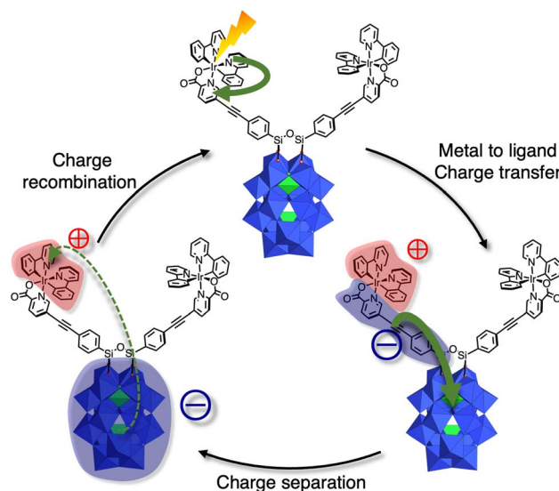
Fig. 5 Directionality in the photoinduced electron transfers of the POM-Ir(III) assembly [P 2 W 17 O 61 {O(SiC 36 H 23 O 2 N 3 Ir) 2 }] 6- , conferred by the heteroleptic character of the Ir(III) complex. The red and blue cloud respectively represent the localization of the positive and negative charges in the different excited states. 51
