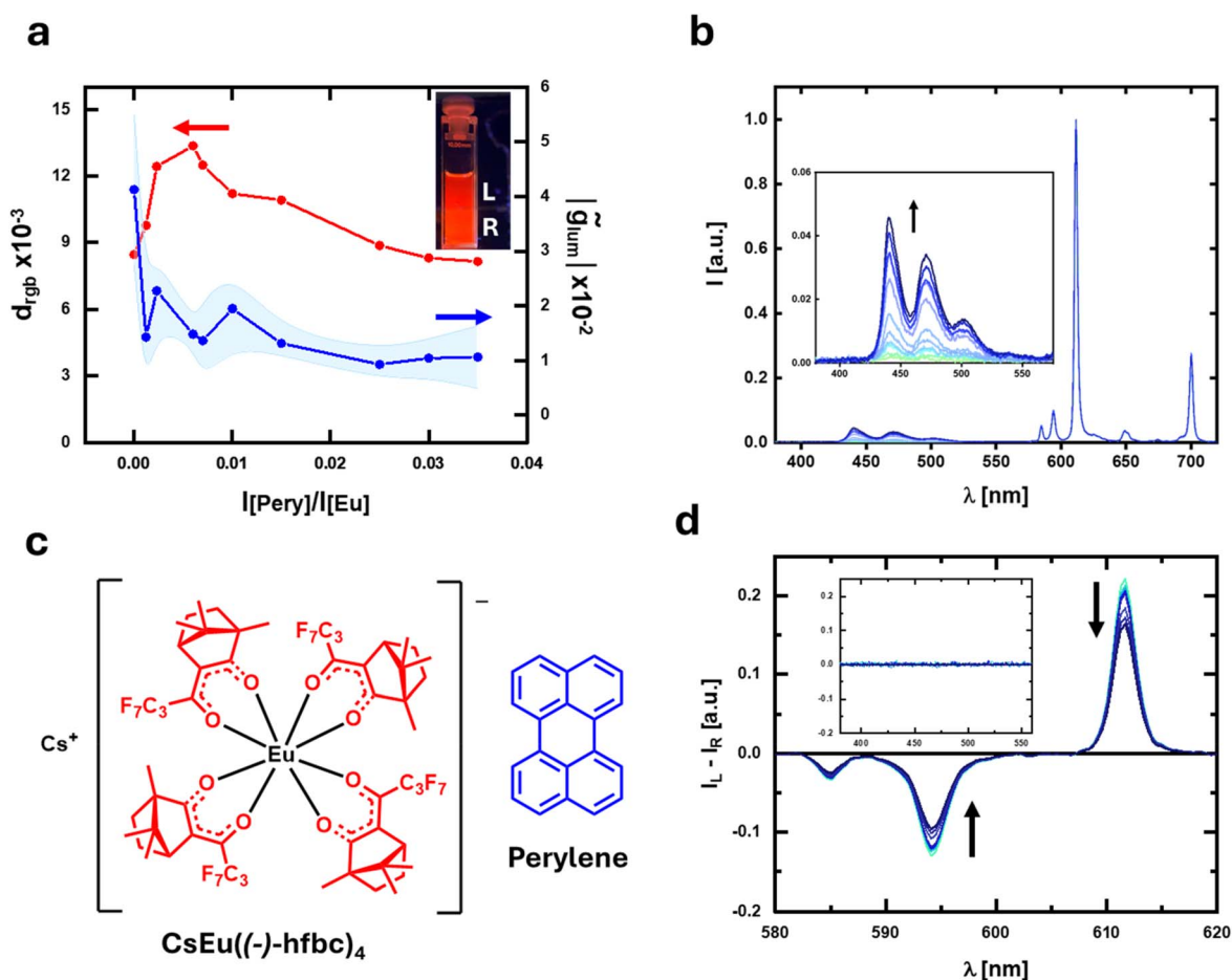
Fig. 3 (a) Plot of d_{\text{rgb}} (red) and \tilde{g}_{\text{lum}} (blue) for a solution of CsEu((-)-hfbc)_4 containing increasing amounts of perylene. Inset: photo of a CsEu((-)-hfbc)_4 /perylene solution irradiated with a 365 nm source, seen through an L and R circular polarizer (upper and lower part of the photo). (b) Emission and (d) corresponding CPL spectra of the solution of CsEu((-)-hfbc)_4 containing increasing amounts of perylene; the CPL spectra are normalized by the integral of the corresponding total emission spectrum. (c) CsEu((-)-hfbc)_4 and perylene.
