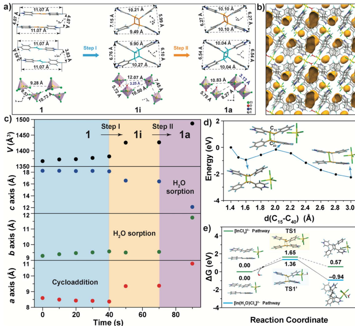
Fig. 2 (a) Geometrical variation of \text{LH}^+ dimers and the [\text{InCl}_5]^{2-} polyhedron in 1 , 1i , and 1a . (b) Schematic illustration of the free volume in 1 (probe radius: 1.0 Å; approx. grid spacing: 0.2 Å). (c) Lattice parameters of 1 at different irradiation times (light source: 450 nm, 260 \text{mW cm}^{-2} ). (d) Energy profile of the [2 + 2] cycloaddition reaction with constrained C–C bond length. The \text{C}_{15} – \text{C}_{40} bond length was fixed during the optimization process to examine the impact of this constraint on the reaction pathway. (e) Computational study of \text{LH}^+ dimers, the [\text{InCl}_5]^{2-} polyhedron, \text{LH}^+ photodimers, and the [\text{In}(\text{H}_2\text{O})\text{Cl}_5]^{2-} octahedron involved in [2 + 2] cycloaddition reactions.
