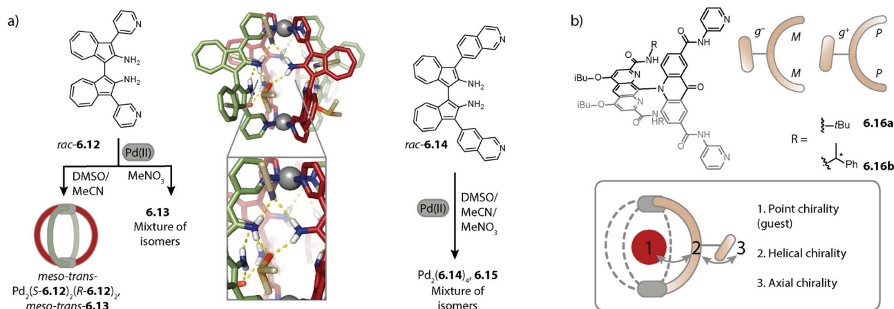
Fig. 28 (a) Solvent dependent chiral social self-sorting with ligand 6.12; the expansion of the X-ray structure shows solvent molecules acting as tethers between two adjacent ligands. (b) Bidirectional transmission of chirality between the cavity and the periphery of the cage.
