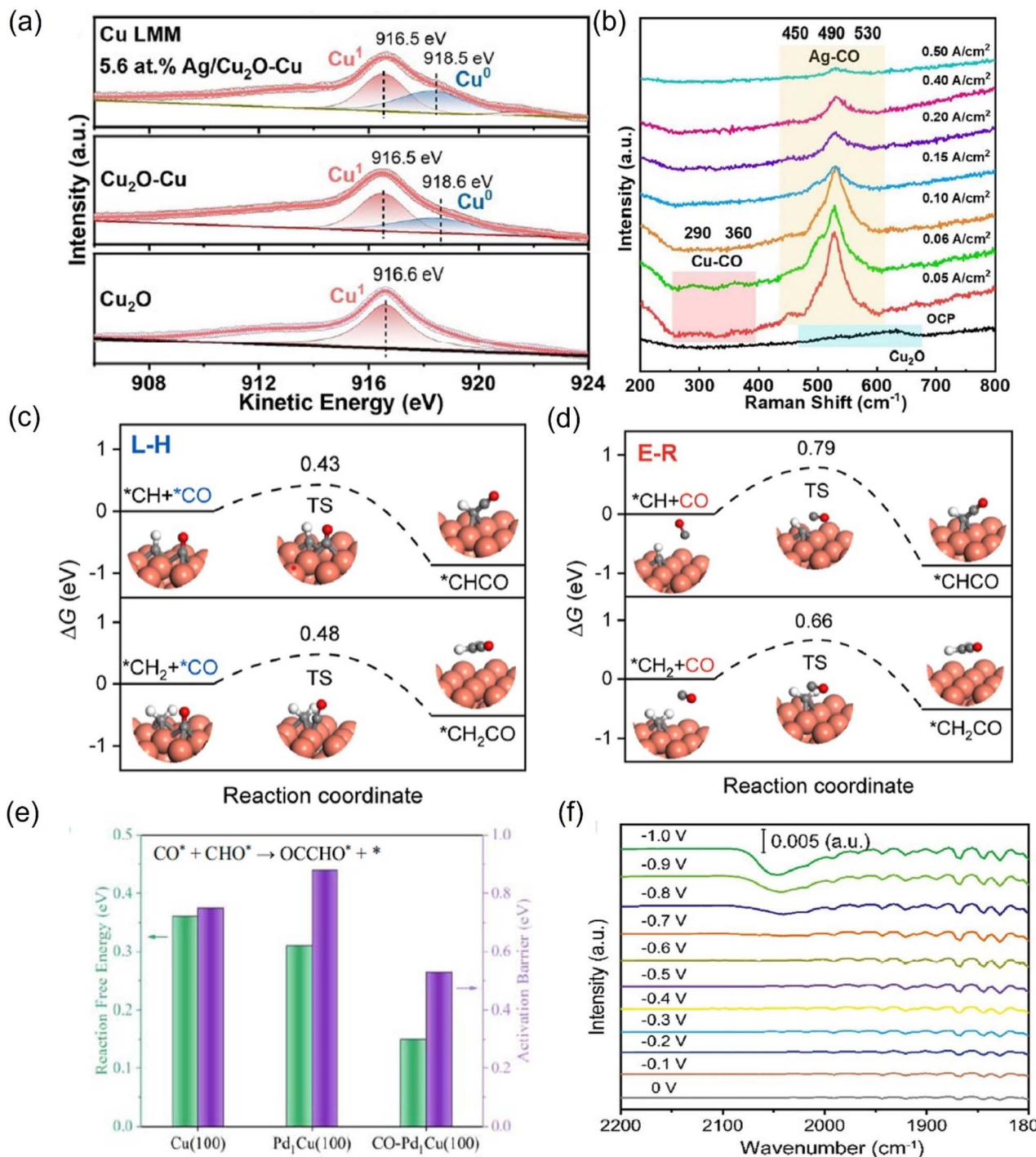
Fig. 11 (a) Cu LMM spectra of Cu 2 O, Cu 2 O-Cu, and 5.6 at.% Ag/Cu 2 O-Cu catalysts. (b) Raman shift of the 5.6 at.% Ag/Cu 2 O-Cu catalyst. DFT calculations: barriers for *CH x ( x = 1, 2 ) coupling with *CO/CO via (c) L-H and (d) E-R mechanisms. (e) The reaction free energies and activation barriers of C-C coupling on Cu (100) and Pd 1 Cu (100). (f) In situ ATR-IR spectra of Au-Cu Janus NSs. (a and b) Reproduced with permission. 144 Copyright 2025, American Chemical Society. (c and d) Reproduced with permission. 146 Copyright 2024, American Chemical Society. (e) Reproduced with permission. 147 Copyright 2023, Springer Nature. (f) Reproduced with permission. 148 Copyright 2022, Wiley-VCH Verlag.
