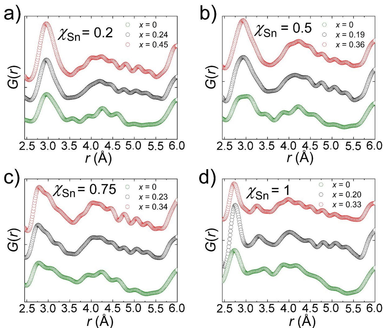
Figure 7: Experimental pair distribution function (PDF) curves for representative compounds in the \text{FA}_{1-x}\text{en}_x\text{Pb}_{\eta-y}\text{Sn}_y\text{Br}_3 family of perovskites in four panels (a, b, c, & d) depending on the experimentally determined Sn fraction ( \chi_{\text{Sn}} ) and ethylenediammonium fraction ( x ). Here the PDF of \text{FASnBr}_3 is plotted from our previous works for comparison. 51
