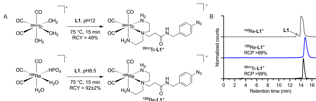
Fig. 4 Radiosynthesis of the \text{M-L1}^+ complexes ( \text{M} = {}^{99\text{m}}\text{Tc}, {}^{188}/{}^{186}\text{Re} ) showing (A) the synthetic procedures employed and (B) (radio-)HPLC chromatograms of ^{99\text{m}}\text{Tc-L1}^+ , ^{188}\text{Re-L1}^+ , and ^{nat}\text{Re-L1}^+ (UV trace, 254 nm).
