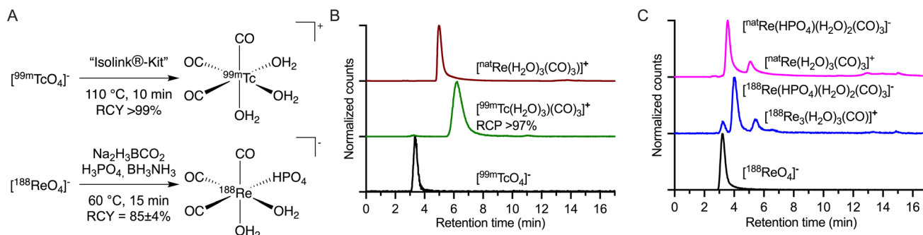
Fig. 1 Chemical reactions for the preparation and chromatographic characterization of \{\text{M}(\text{CO})_3\}^+ ( \text{M} = ^{99m}\text{Tc} , ^{188}\text{Re} or \text{natRe} ) species. (A) Radiosynthesis of [^{99m}\text{Tc}(\text{H}_2\text{O})_3(\text{CO})_3]^+ and [^{188}\text{Re}(\text{HPO}_4)(\text{H}_2\text{O})_2(\text{CO})_3]^- (please see ESI Schemes S1 and S2 and Fig. S1 and S2 for further details†); (B) radio-HPLC chromatograms of [^{99m}\text{TcO}_4]^- (black radiotracer), [^{99m}\text{Tc}(\text{H}_2\text{O})_3(\text{CO})_3]^+ (green radiotracer), and [\text{natRe}(\text{H}_2\text{O})_3(\text{CO})_3]^+ (red, electronic absorption trace 254 nm). (C) Equivalent radio-HPLC chromatograms obtained during the synthesis of the \{\text{natRe}(\text{CO})_3\}^+ core showing the retention times of the parent [^{188}\text{ReO}_4]^- (black radiotracer), the ^{188}\text{Re} -reaction mixture (blue radiotracer), and the mixture formed by using [\text{natRe}(\text{H}_2\text{O})_3(\text{CO})_3]^+ (magenta electronic absorption trace 254 nm) placed under the experimental conditions used in the ^{188}\text{Re} radiochemistry. Discrete peaks for [^{188}\text{Re}(\text{HPO}_4)(\text{H}_2\text{O})_2(\text{CO})_3]^- and [\text{natRe}(\text{H}_2\text{O})_3(\text{CO})_3]^+ were observed at 4.0 min and 5.5 min, respectively.
