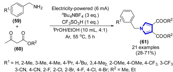
Scheme 16 Synthesis of poly-substituted pyrroles using electro-oxidative intermolecular annulation.
