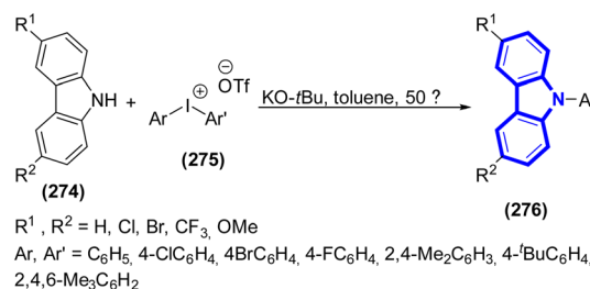
Scheme 74 Synthesis of N -arylcabazoles using diaryliodonium salts.
