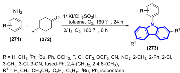
Scheme 73 Synthesis of N -arylcabazoles using transition metal-free one-pot reaction.
