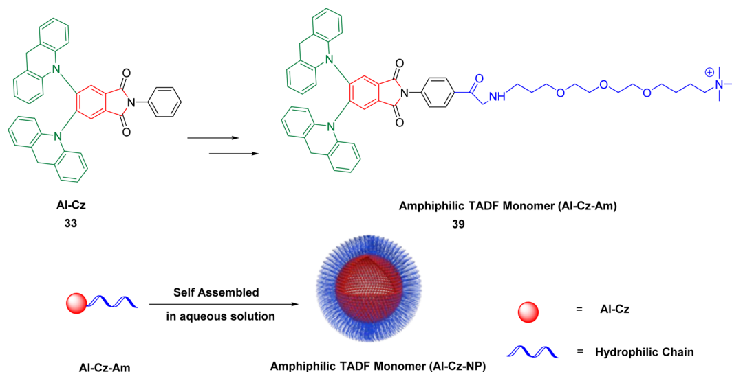
Fig. 17 Structure of amphoteric TADF monomer 39 and the synthesis of TADF nanoprobe AI-Cz-NP. Reproduced from ref. 163 with permission from the Royal Society of Chemistry.
