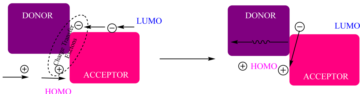
Fig. 5 Electrically excited generation of exciplexes.
