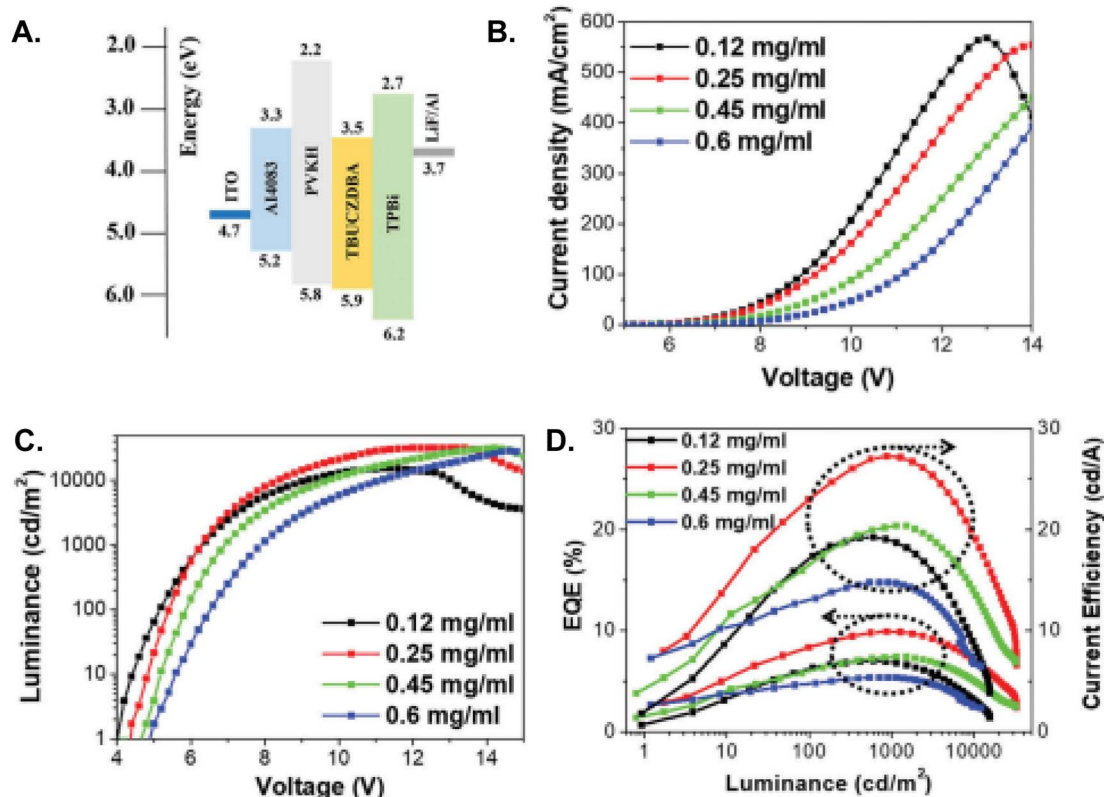
Fig. 82 Characterization of OLED device with different thicknesses of inkjet printed t\text{BuCzDBA} film as the active layer (A) device architecture and energy level diagram of the prepared OLEDs (B) current density versus voltage, (C) luminance versus voltage, and (D) efficiency versus luminance characteristics.
