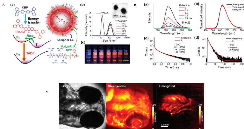
Fig. 24 (A) Representation of TPAAQ/CBP/CPG TADF nanoparticles (b) DLS histograms showing the size of the nanoparticles and inset TEM images showing their morphology. (c) Photographs of the nanoparticle solutions under UV irradiation. (B) Time-gated emission spectra of the nanoparticles at various delay times. (C) Imaging of zebrafish incubated with TPAAQ/CBP/CPG nanoparticles, where the bright field is displayed on the left side of the figure, the steady-state luminescence is shown in the middle, and the time-gated luminescence is displayed on the right. Reproduced from ref. 173 with permission from John Wiley & Sons, Copyright © 2024, Wiley-VCH Verlag GmbH & Co. KGaA, Weinheim.
