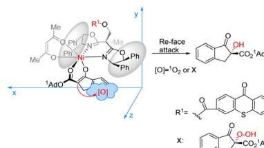
Fig. 17 Stereoinduction model of asymmetric \alpha -hydroxylation catalyzed by complexation of ketone C17 with Ni ( \text{acac} ) 2 .
