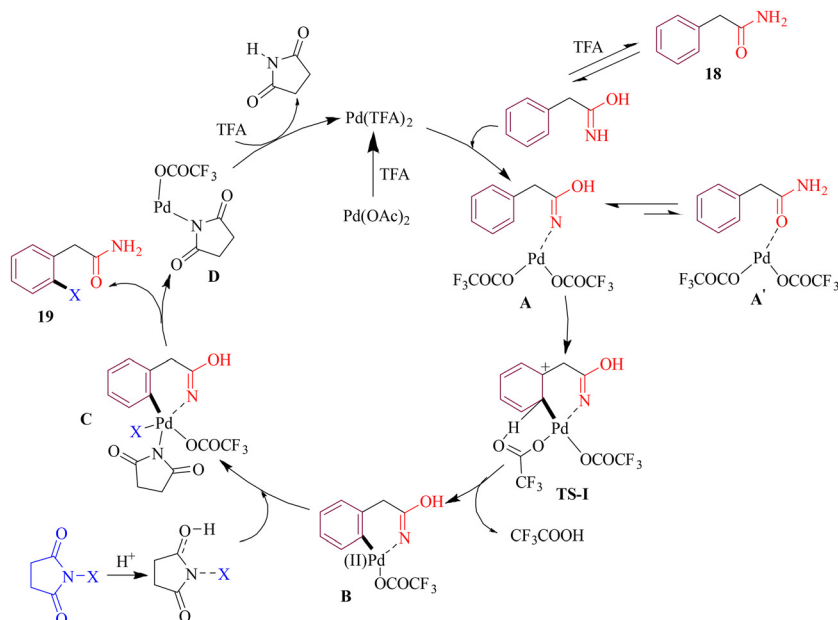
Scheme 9 Palladium-catalyzed ortho C–H bromination/iodination of aliphatic amides.
